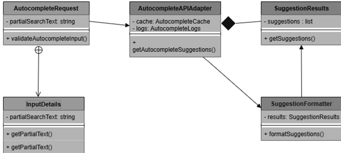
Autocomplete API Adapter – Class Diagram
